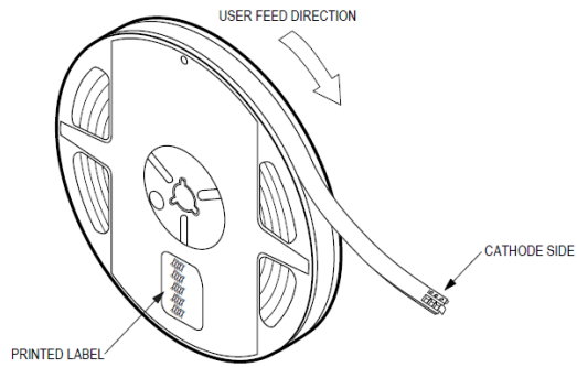
Figure 7. Reel orientation
